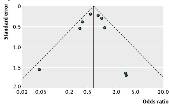
Funnel plot for the meta-analysis of the short term safety (periprocedural mortality or stroke) of carotid endarterectomy compared with carotid artery stenting
